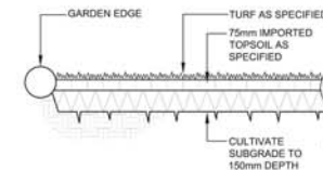
3 TURF SECTION 1:20
