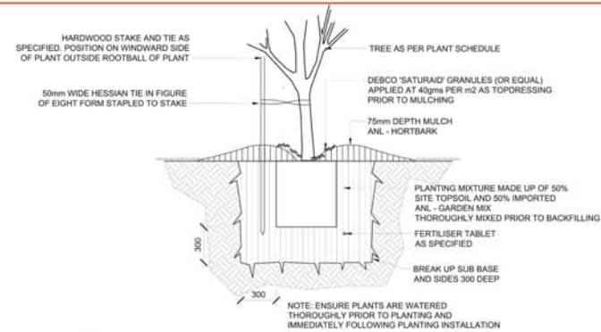
1 TREE PLANTING TYPICAL SECTION 1:20
